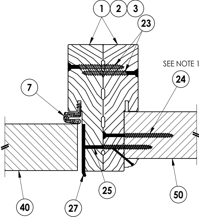
2 HORIZONTAL CROSS SECTION 6 Outswing Shown (Inswing Similar)
