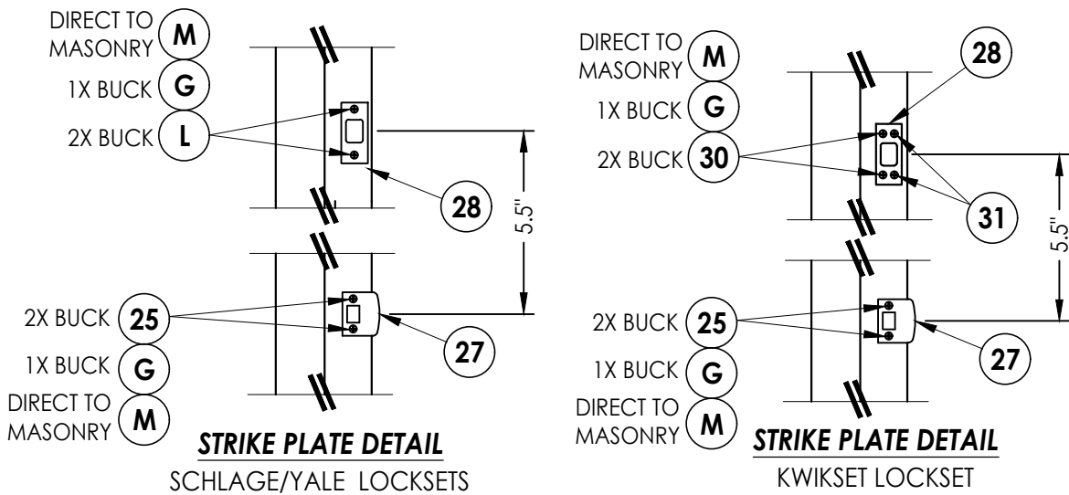
LATCH & DEADBOLT STRIKE PLATE DETAILS
