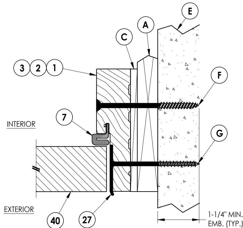
3 8 HORIZONTAL CROSS SECTION Outswing Shown (Inswing Similar) Shown w/ 1X Buck
