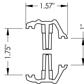
4A TRIMLITE LITE FRAME POLYPROPYLENE
